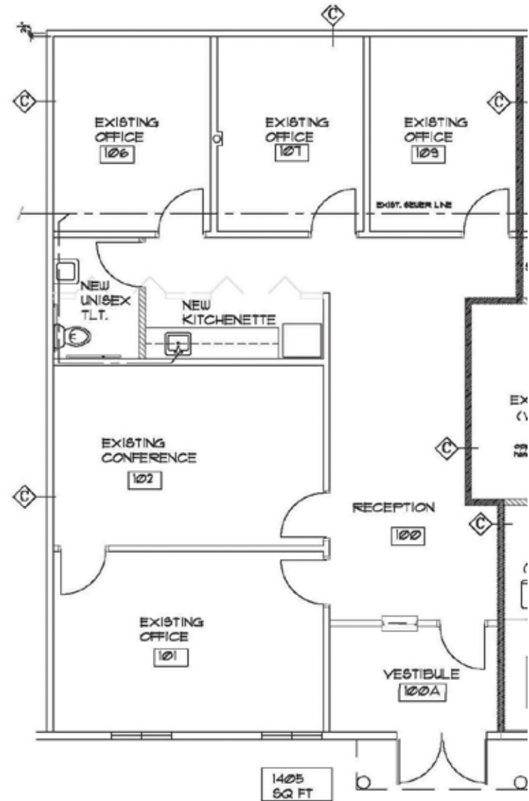
SUITE 114 FLOOR PLAN
